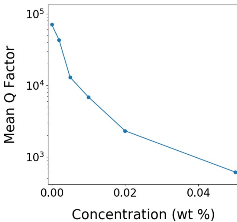
Figure 2: Quality factor as a function of dopant concentration.
