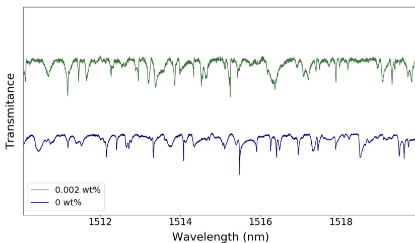
Figure 1: Transmittance spectra of the undoped (blue) and doped (green) resonators
